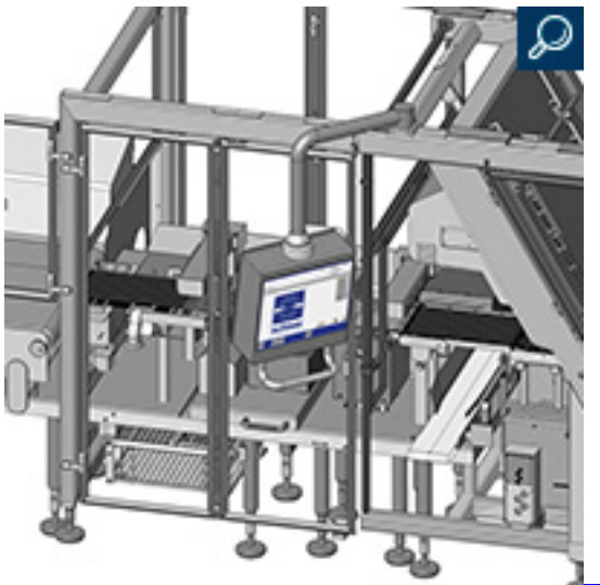
Cured Ham Slicing Lines
